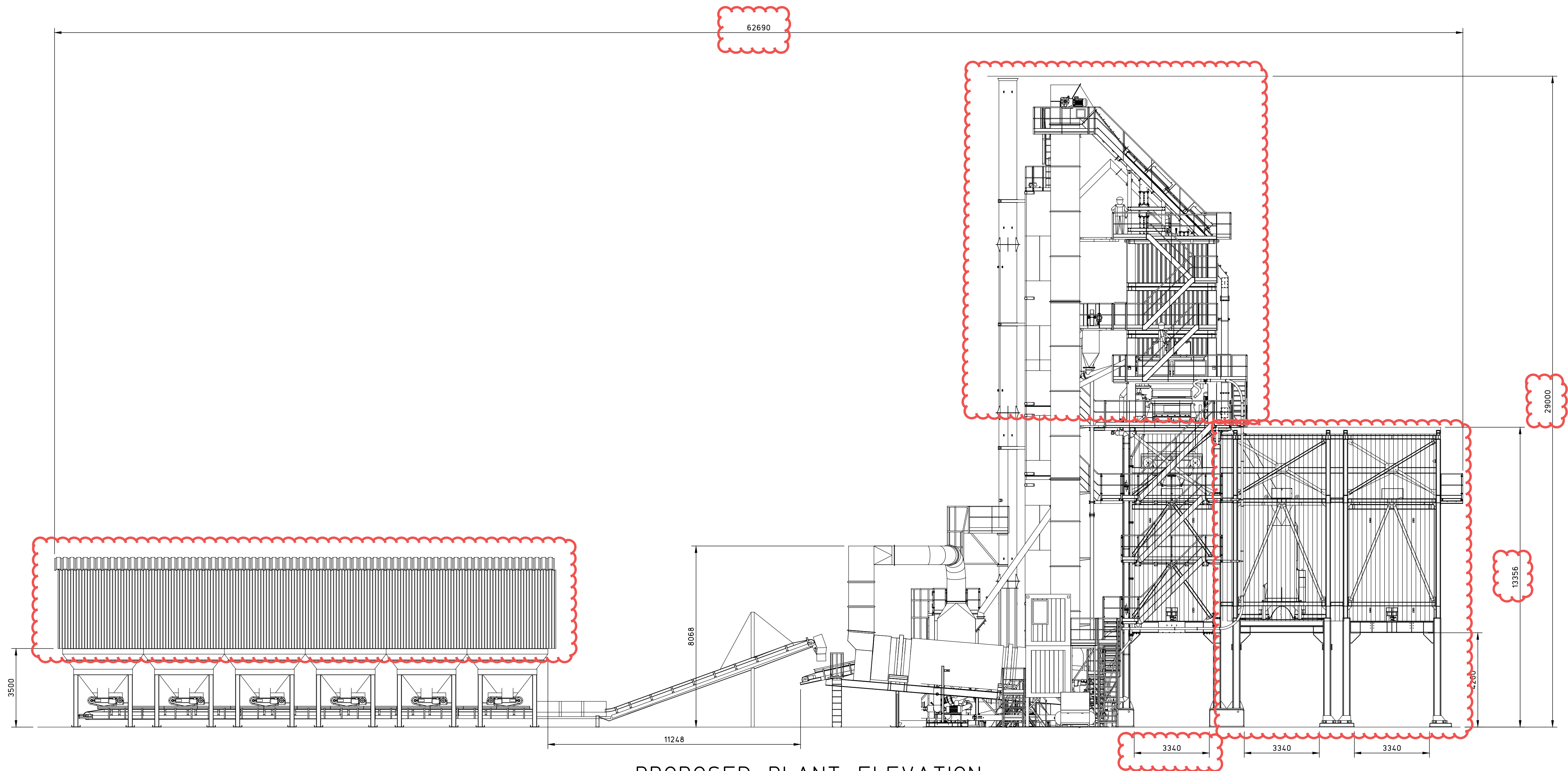
PROPOSED PLANT ELEVATION SCALE 1:100
